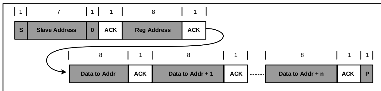
Figure 14: Multi-Write
