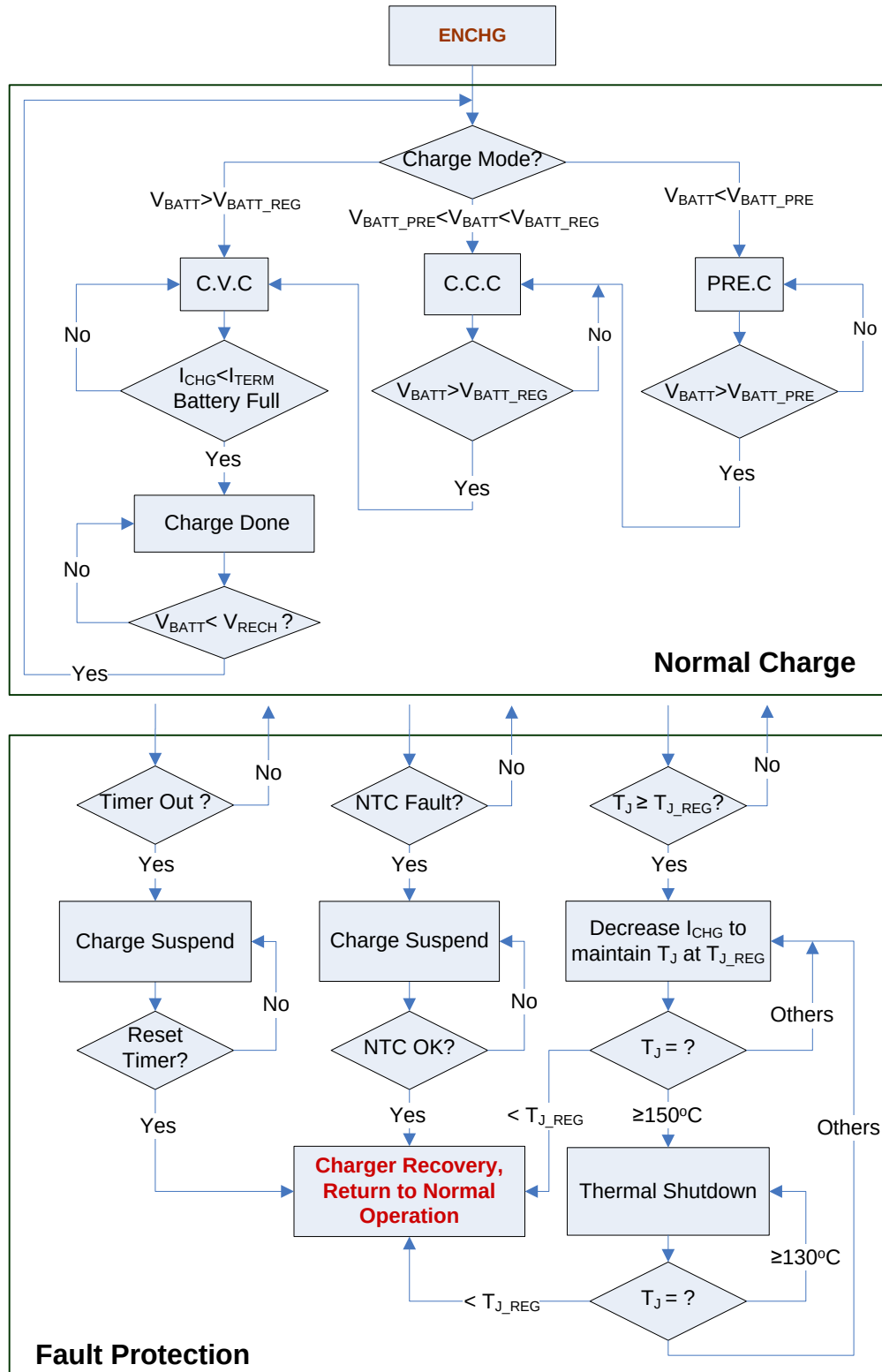
Figure 19: Charging Process
