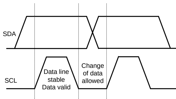
Figure 9: Bit Transfer on the I 2 C Bus
