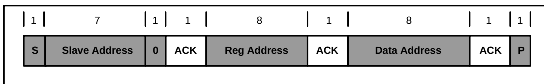
Figure 12: Single Write
