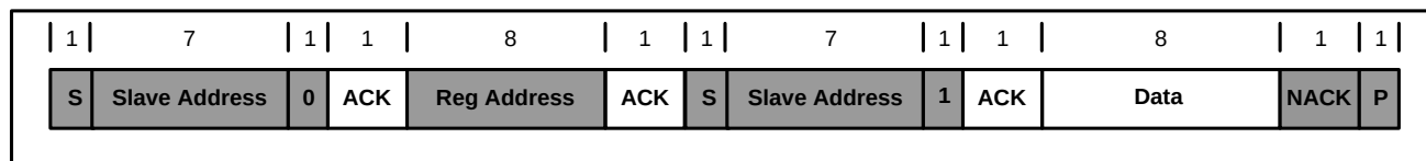
Figure 13: Single Read
