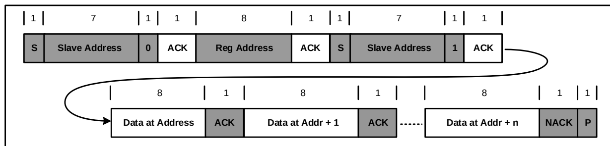
Figure 15: Multi-Read
