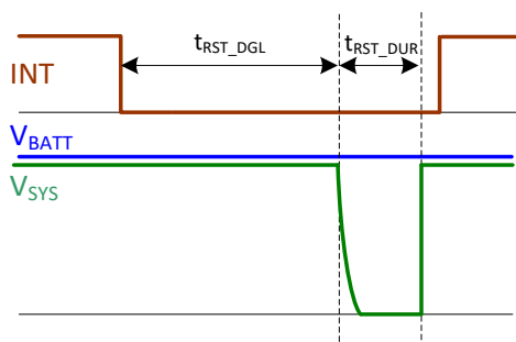
Figure 7: System Reset Function Operation Profile
