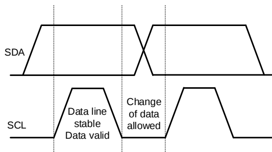
Figure 11: Bit Transfer on the I 2 C Bus
