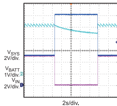
Input Voltage Clamp @ 4.75V Charge Mode
