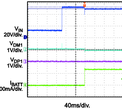
USB Insertion, No Load Connection
