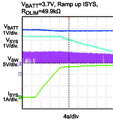
Boost Mode CC Function
