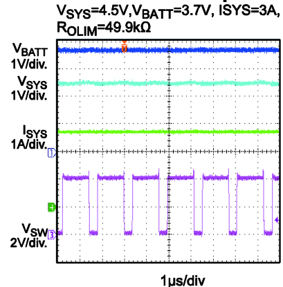
Boost Mode CC Operation
