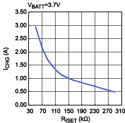
Programmable Charge Current, Charge Mode
