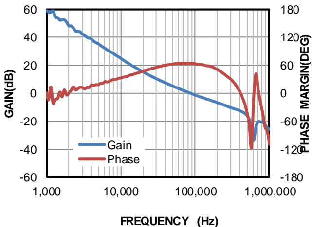
Bode Plot
