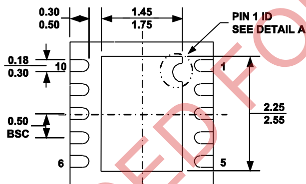
QFN10 (3mm x 3mm)
