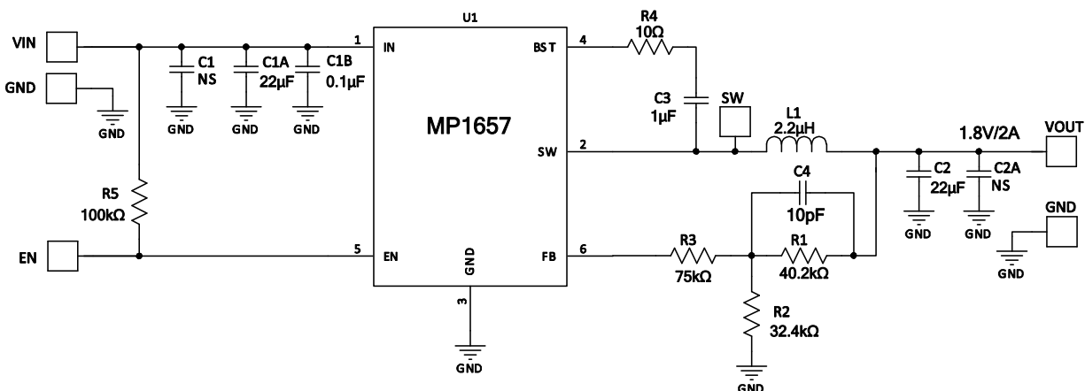
Figure 9: 12VIN, 1.8V/2A Output
