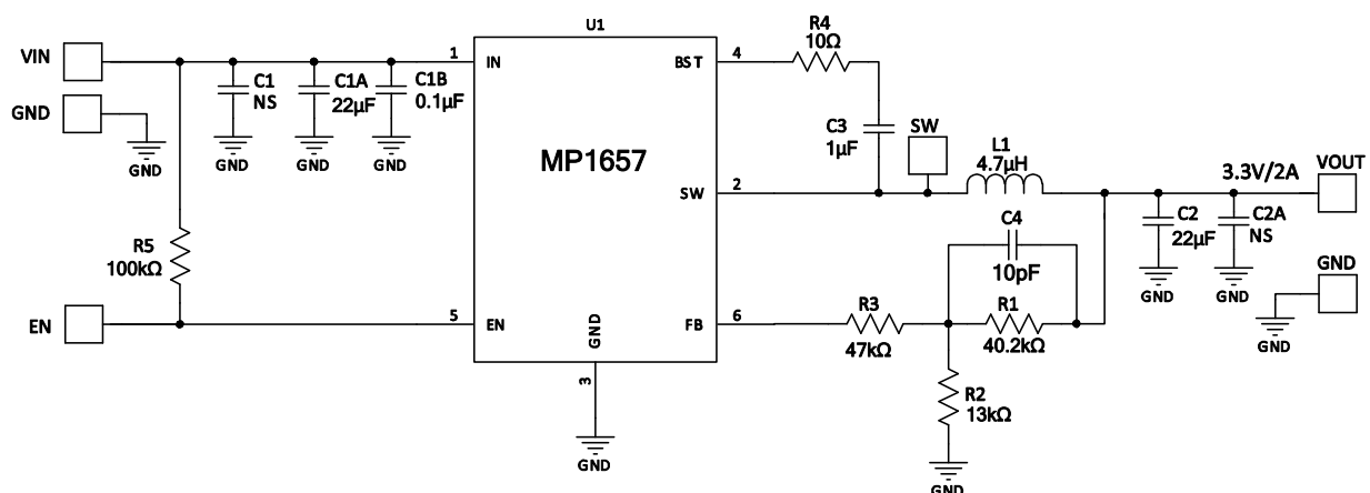
Figure 7: 12VIN, 3.3V/2A Output
