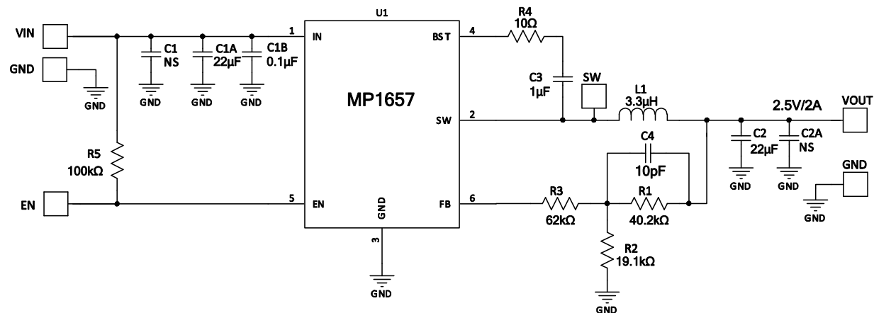
Figure 8: 12VIN, 2.5V/2A Output
