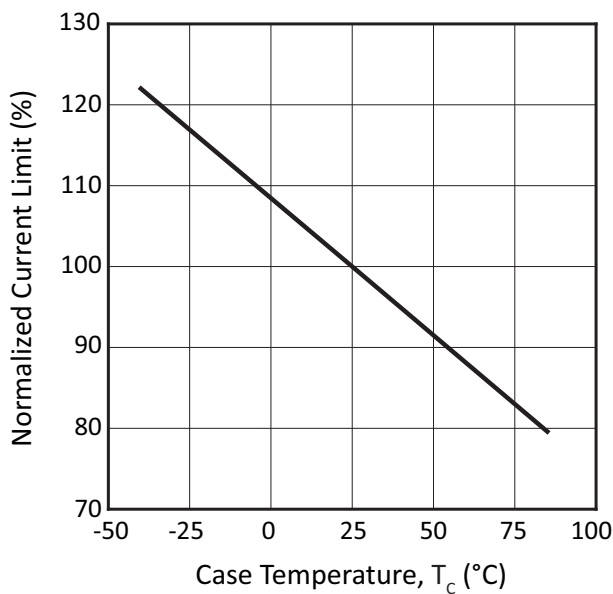
Figure 10: Current Limit
