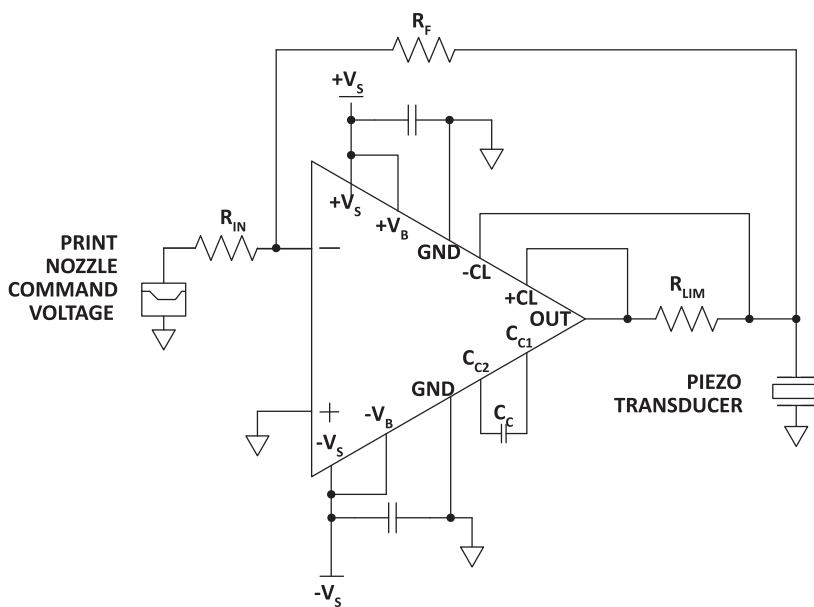
Figure 16: Typical Application
