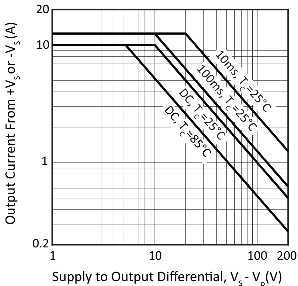
Figure 15: SOA
