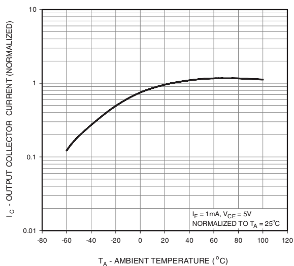
Fig. 3 Output Current vs. Ambient Temperature
