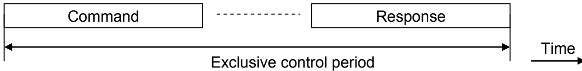
Figure 8-1 Exclusive Control Period
