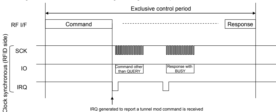
Figure 8-3 Exclusive Control in Tunnel Mode (Clock Synchronous)
