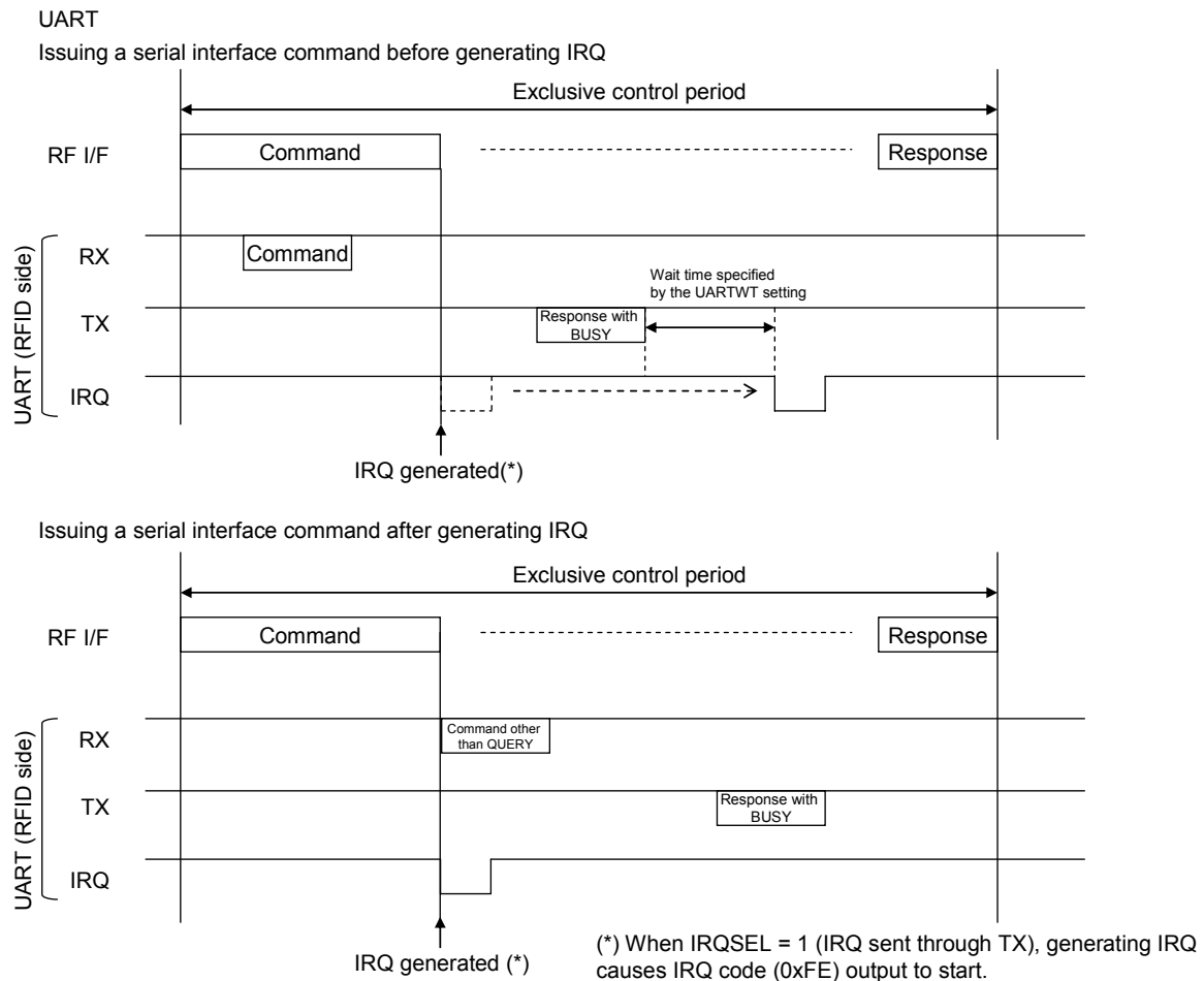
Figure 8-2 Exclusive Control in Tunnel Mode (UART)
