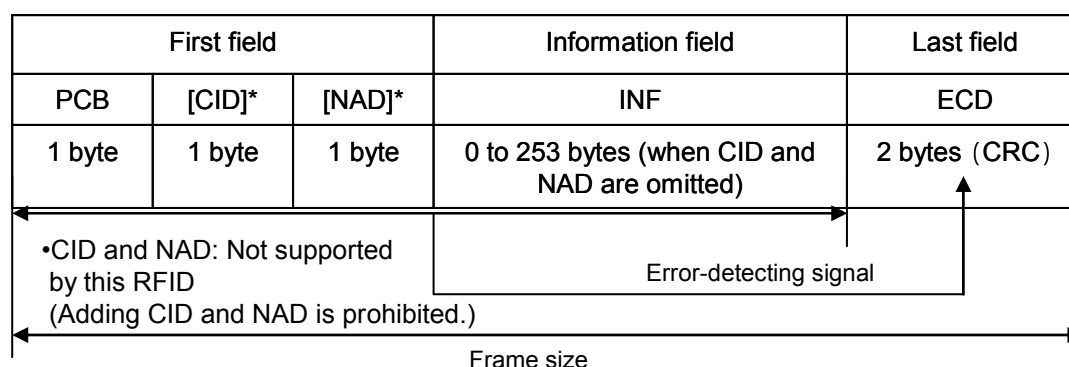
Figure 4-14 ISO/IEC14443-4 Block Format
