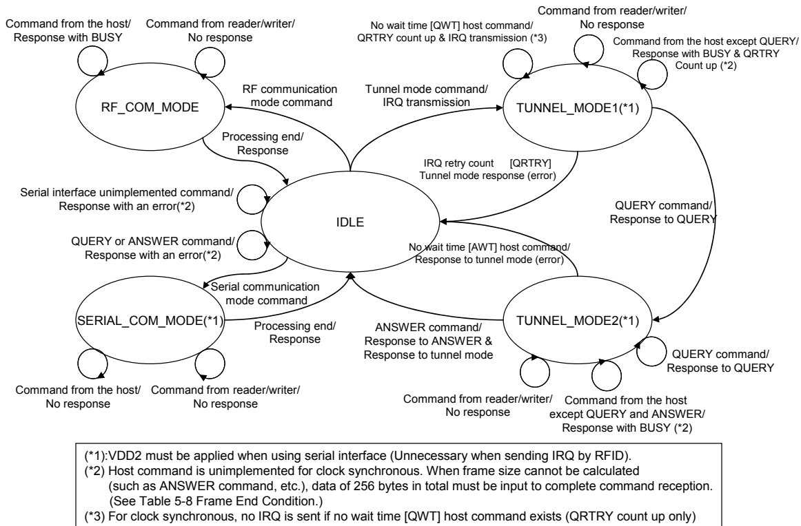
Figure 8-4 State Transition Diagram in Operation Mode
