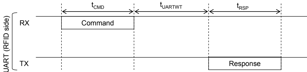
Figure 8-7 Command Processing Time
