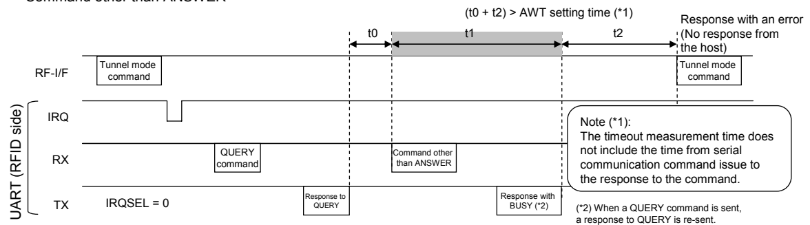
Figure 6-10 Timeout of Waiting for ANSWER Command (Command Other than ANSWER)
