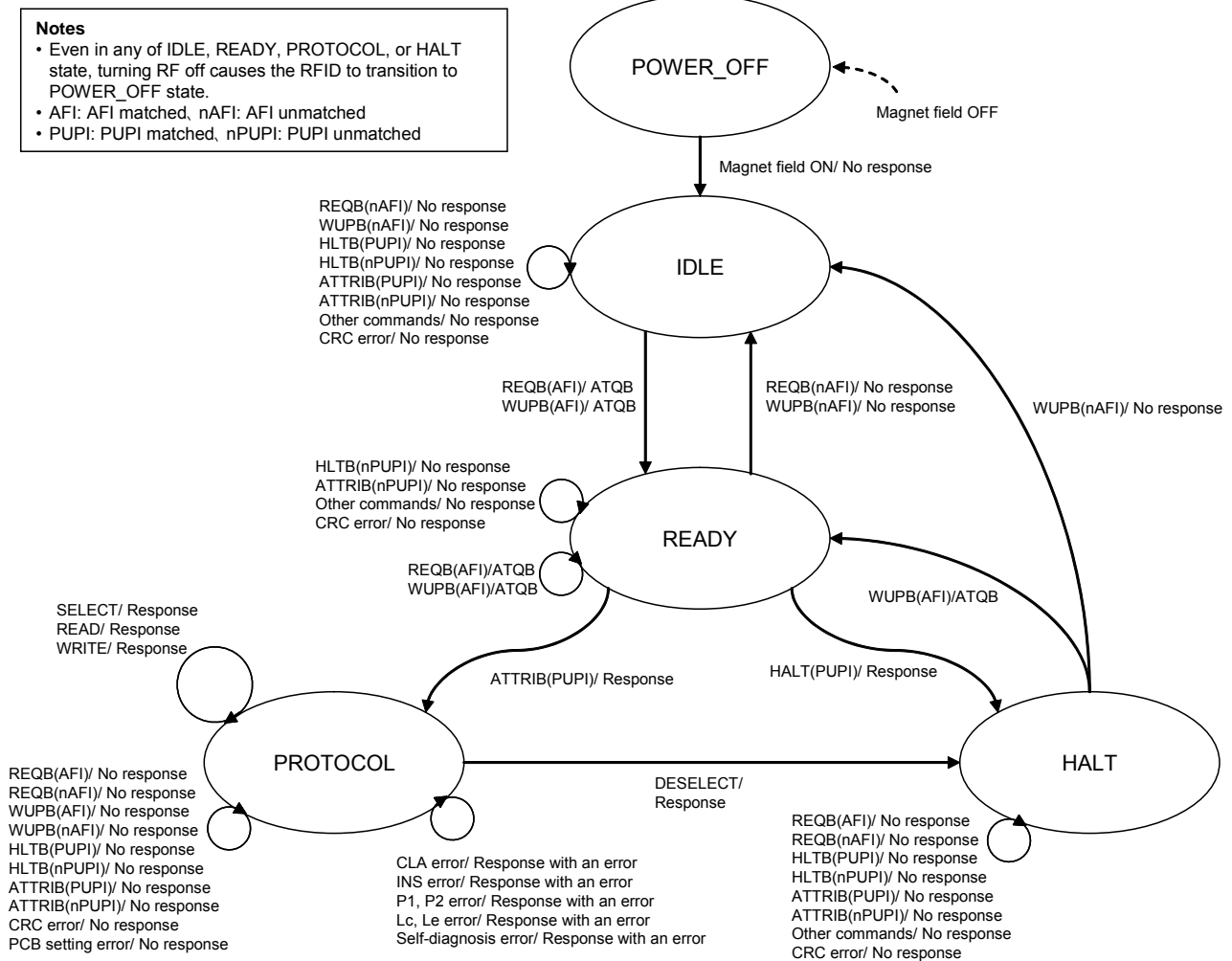
Figure 4-20 State Transition Diagram for Operation Based on ISO/IEC14443 TypeB
