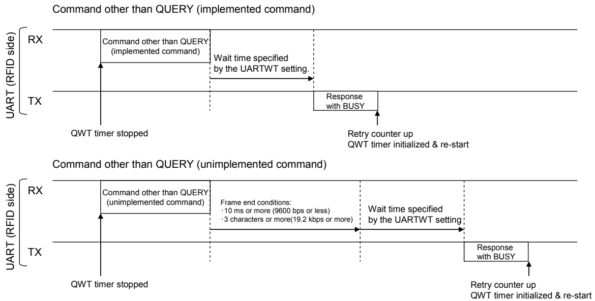
Figure 8-6 Sequence during Command Reception except TUNNEL_MODE1 QUERY (UART only)
