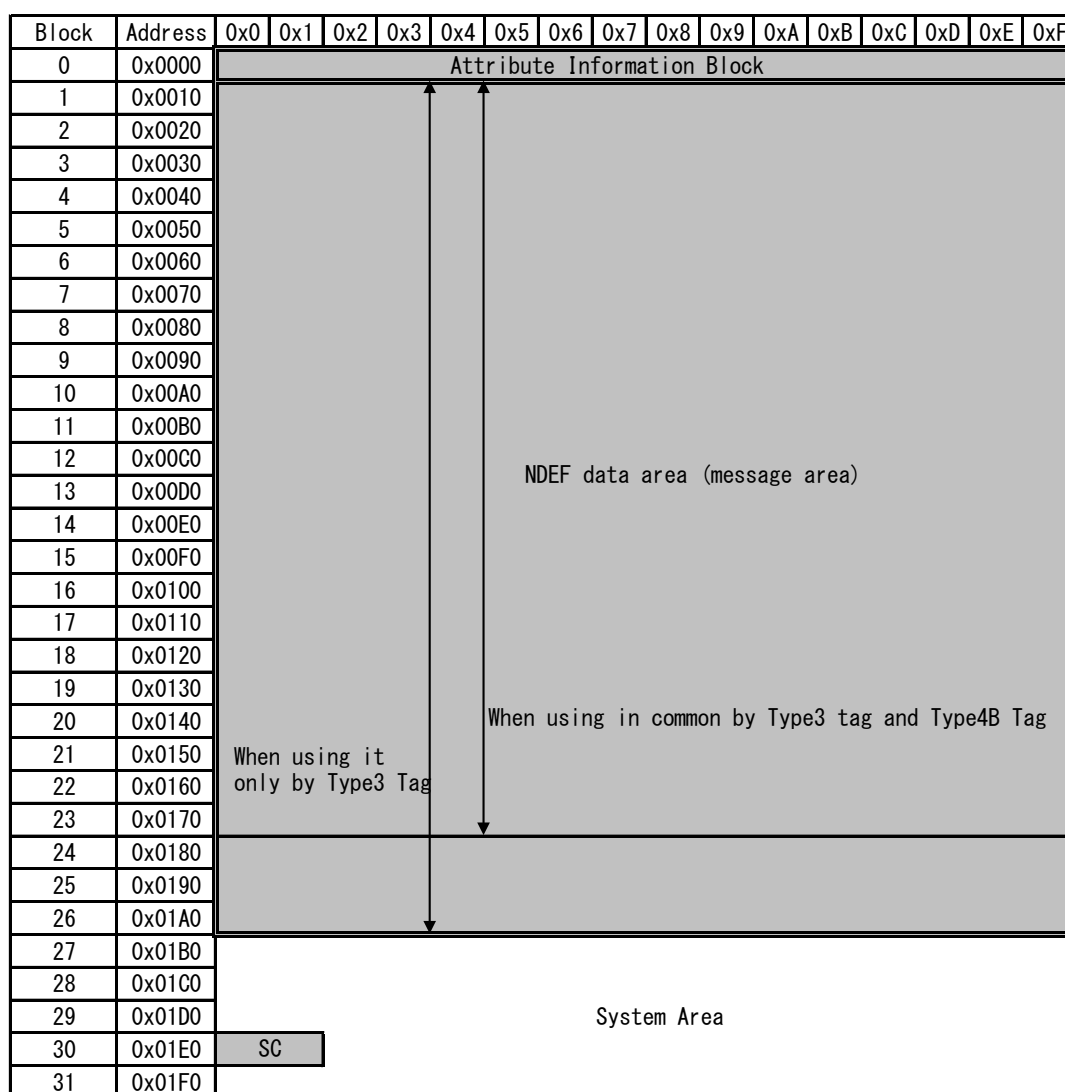
Fig 4-13 The memory map at the time of NDEF use. (NFC Forum Type3 Tag)
