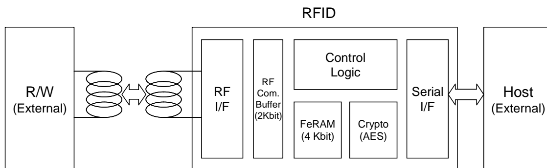
Figure 1-1 Block Diagram
