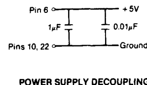
POWER SUPPLY DECOUPLING
