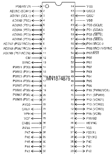
SDIP064-P-0750
