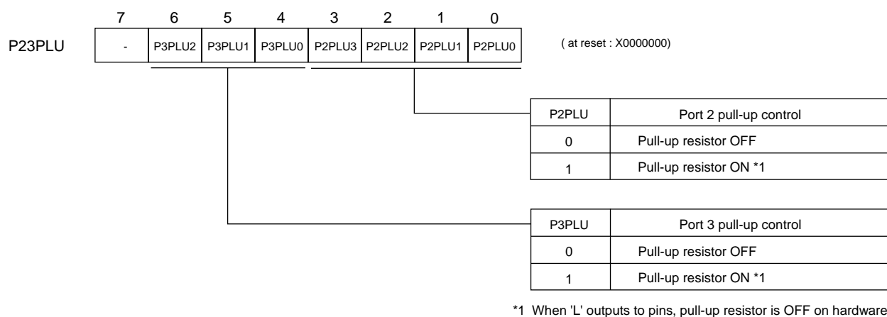
Port 2, Port 3 Pull-up Resistor Control Register (P23PLU : x'022', R/W)
