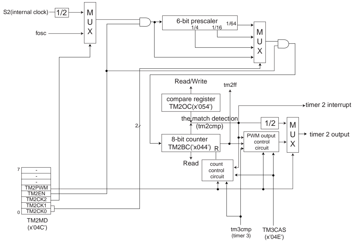
Figure 5-1-1 Timer 2 Block Diagram
