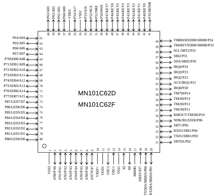
LQFP080-P-1414A *Lead-free
