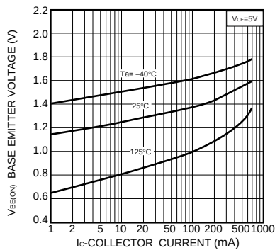
Fig.7 Base emitter "ON" voltage vs collector current
