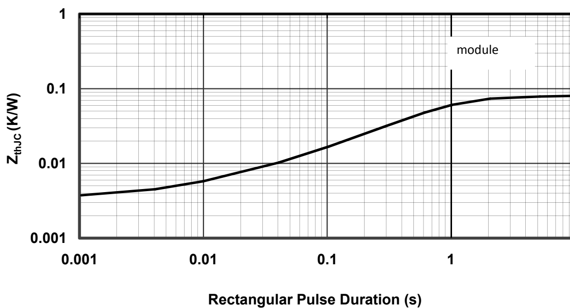
Figure 5. Transient Thermal Impedance
