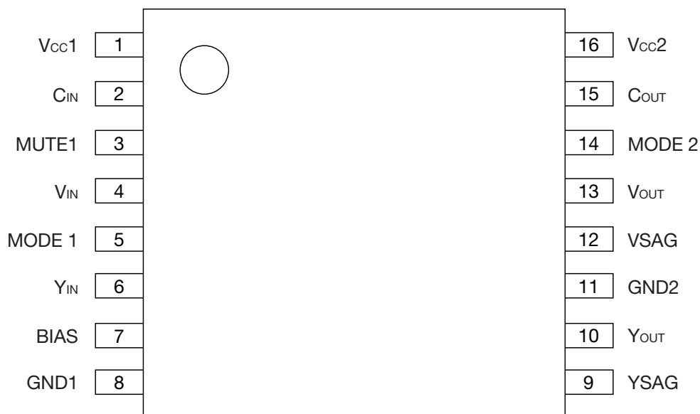
SOP-16C
