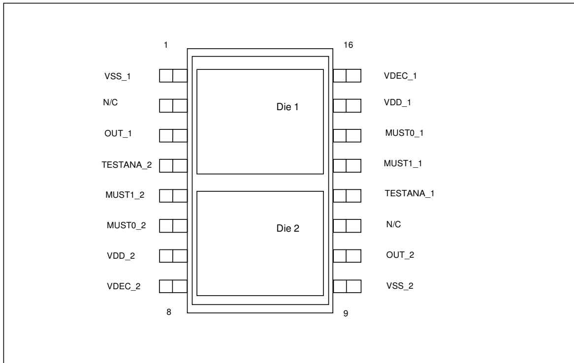
Figure 12: Pinnout
