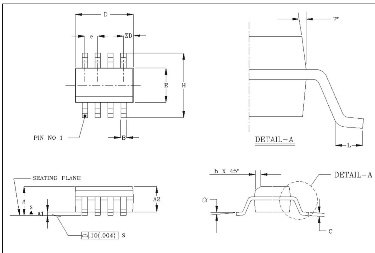
Figure 18: SOIC8 Drawing
