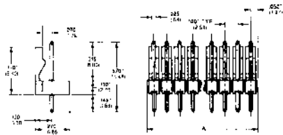
LOCKING HEADER STRAIGHT POST
