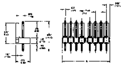
POLARIZING HEADER STRAIGHT POST
