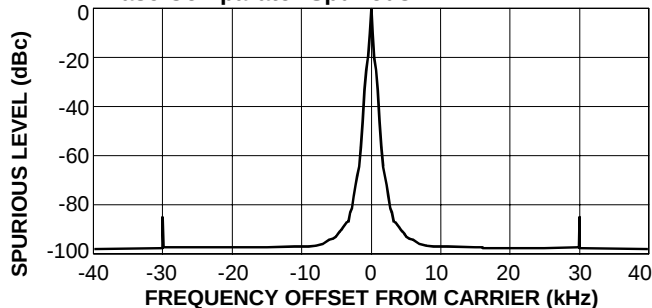
Phase Comparator Spurious
