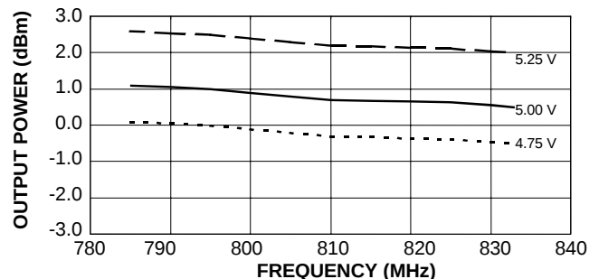
Output Power vs Supply Voltage (V CC1 )
