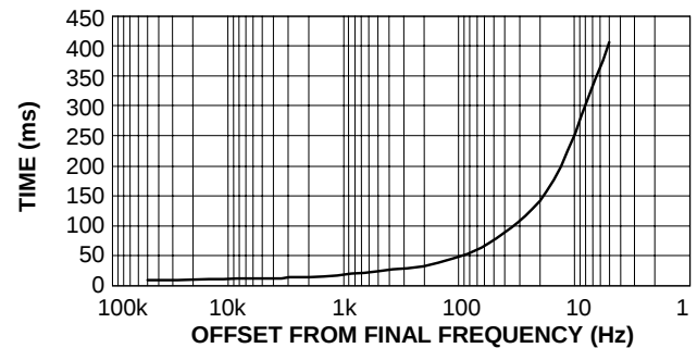
Full Band Switching Time
