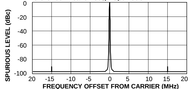
Reference Breakthrough Spurious
