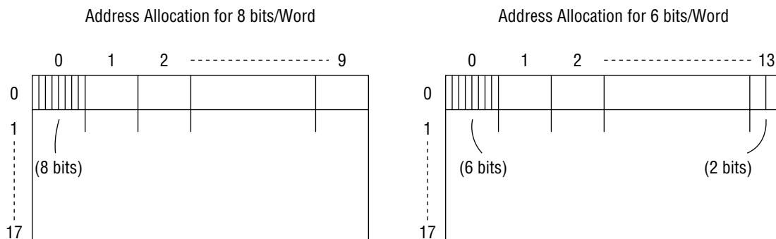
Figure 3 Display Memory Addresses
