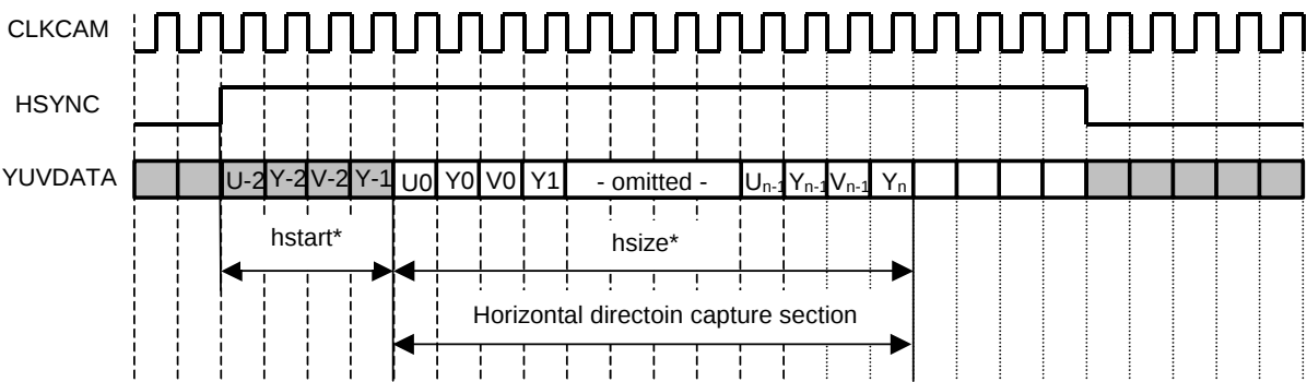
Timing in the horizontal direction
