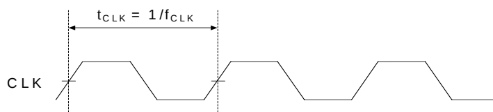
Figure 5-2 Clock Timing
