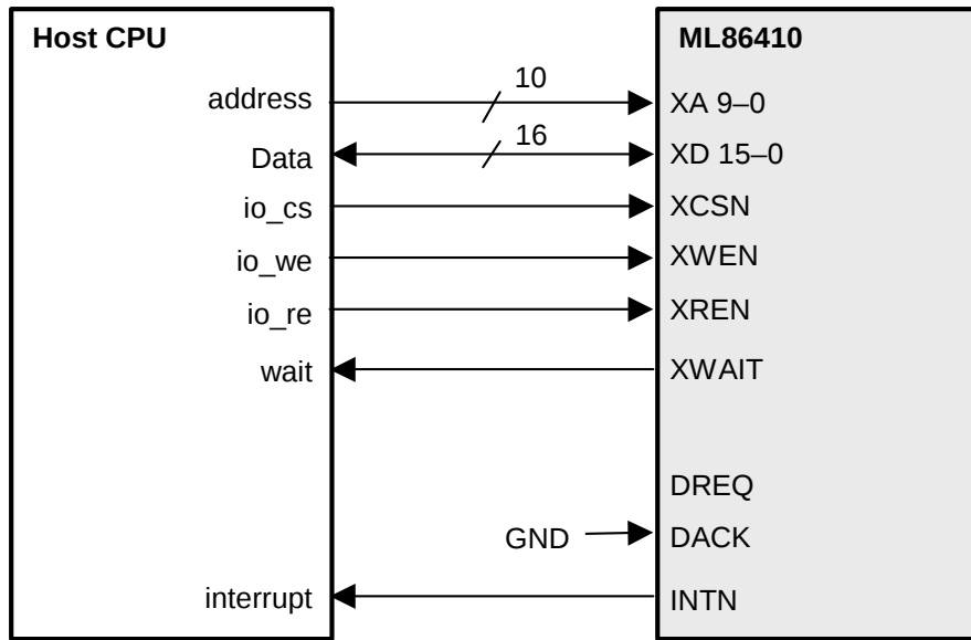
Figure 4-17 Host CPU Connection Example (DMA Signal Control Register Used)
