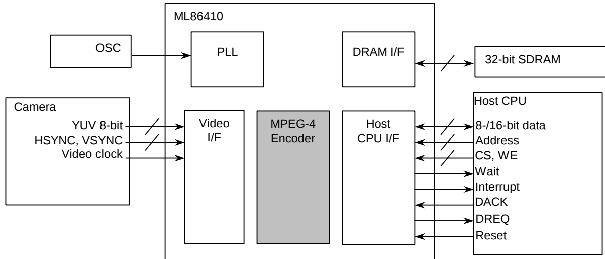
Figure 1-1 Block Diagram
