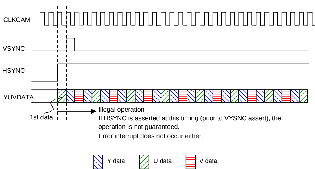
Figure 4-10 Illegal Operation 1 in VSYNC Edge Mode
