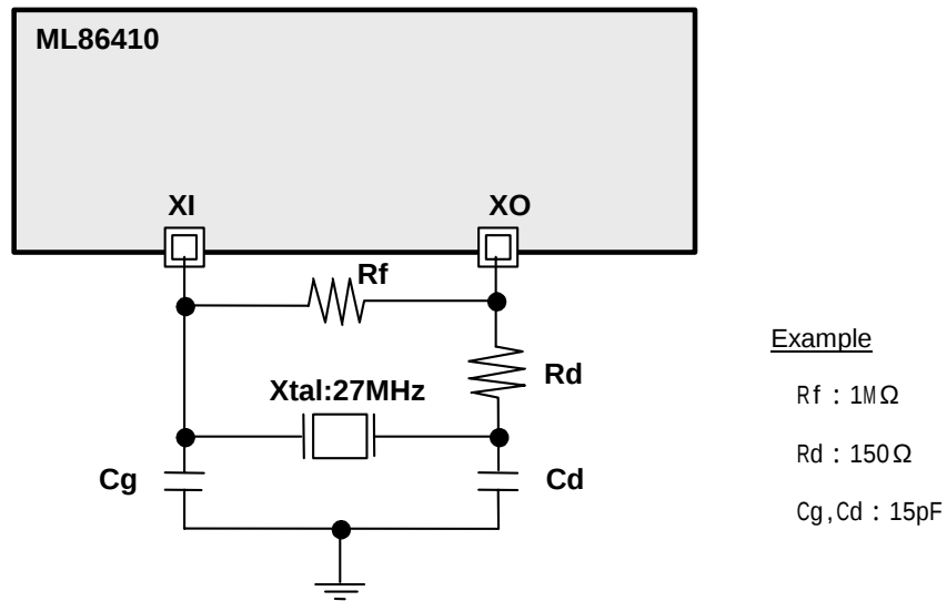
Figure 4-19 Example of External Oscillator Connection
