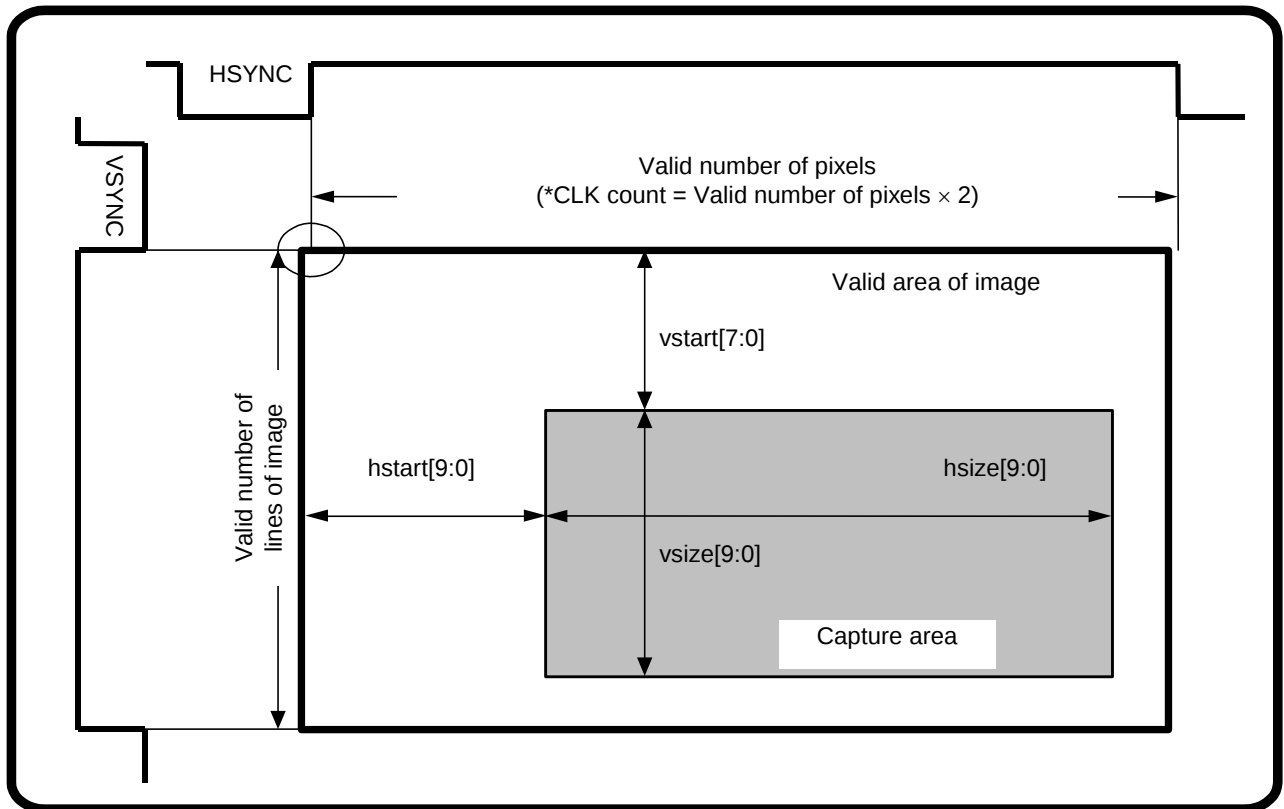
Figure 4-7 Capture Area Detection Conditions
