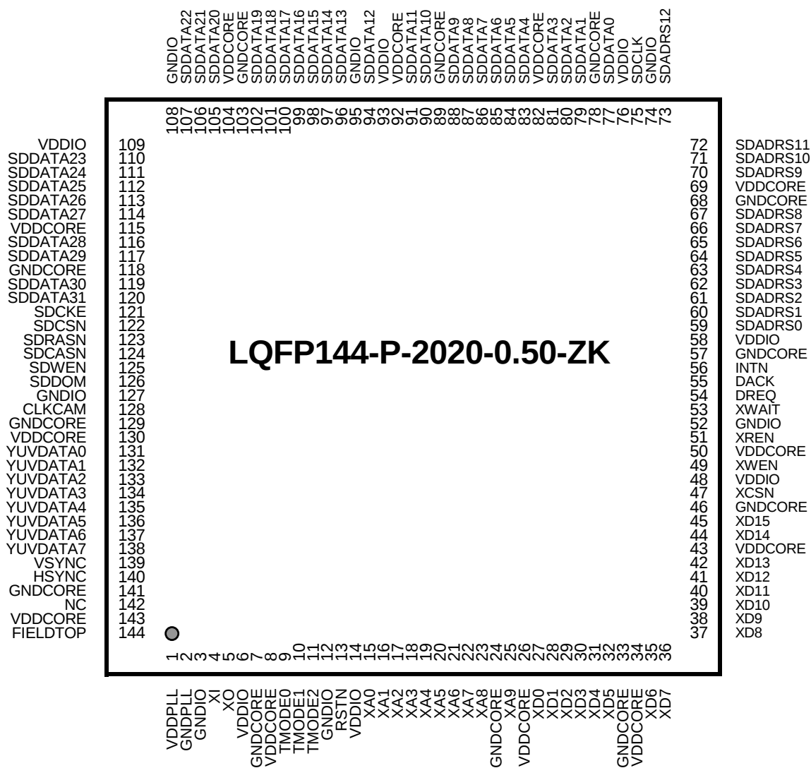
Figure 1-2 144-Pin LQFP Pin Configuration
