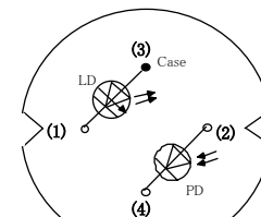
ML725C45F Pin Connection ( Top view )
