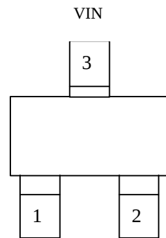
VSS VOUT SOT-23 (Top View)
