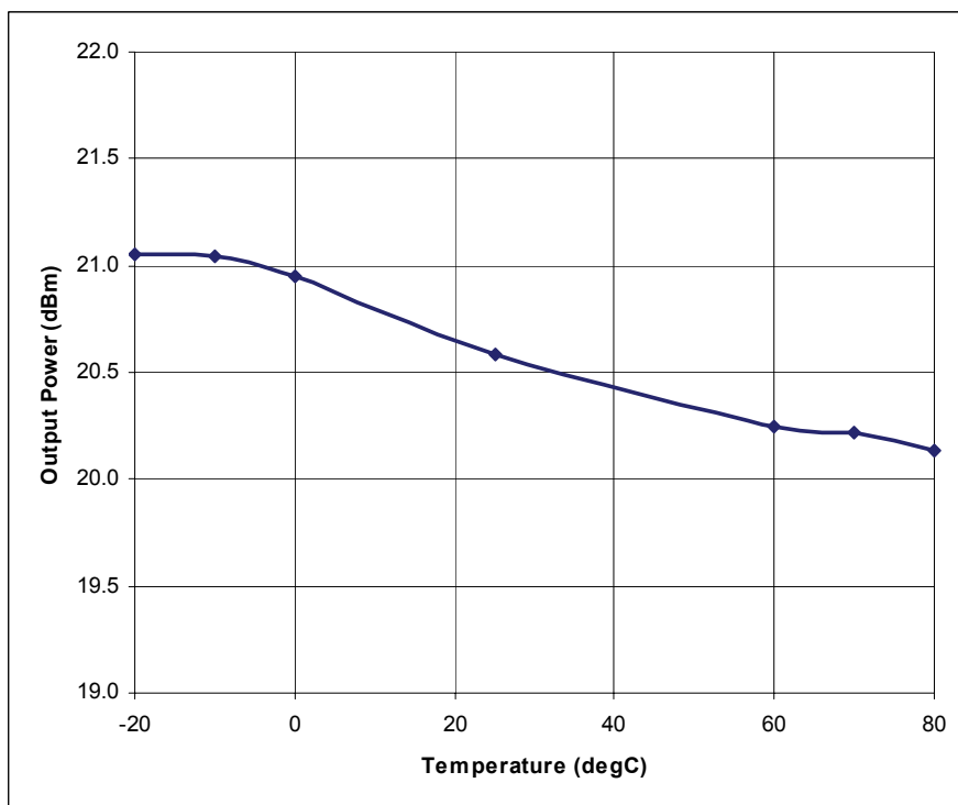
Figure 12 Transmit Power .vs. Temperature
