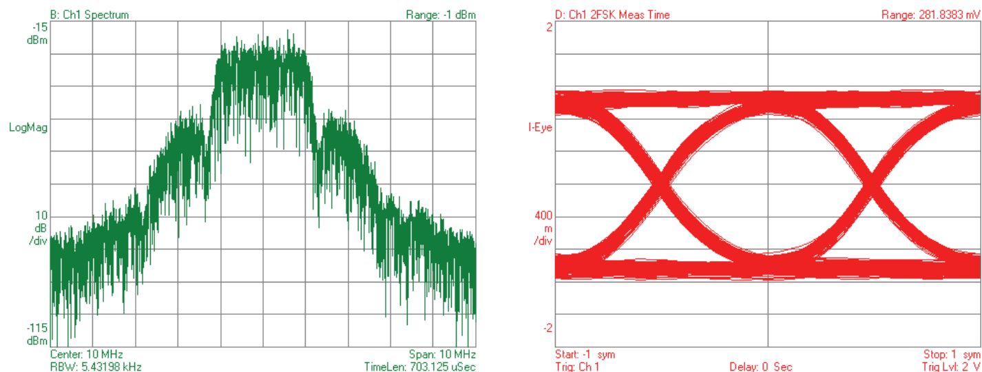
Figure 3 TX output spectrum and eye diagram for 2.048Mbps, PN20 digital mode.
