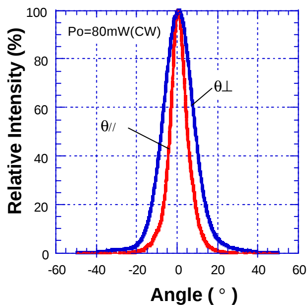
Far-Field-Patterns
