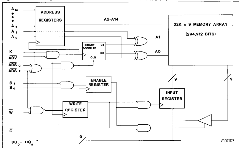
Figure 2. Block Diagram
