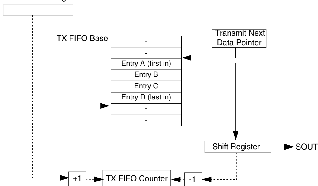
Figure 43-100. TX FIFO Pointers and Counter
