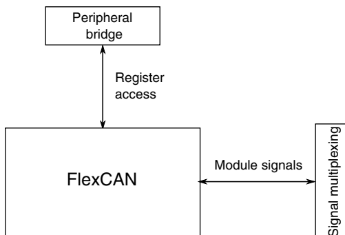
Figure 3-49. CAN configuration
