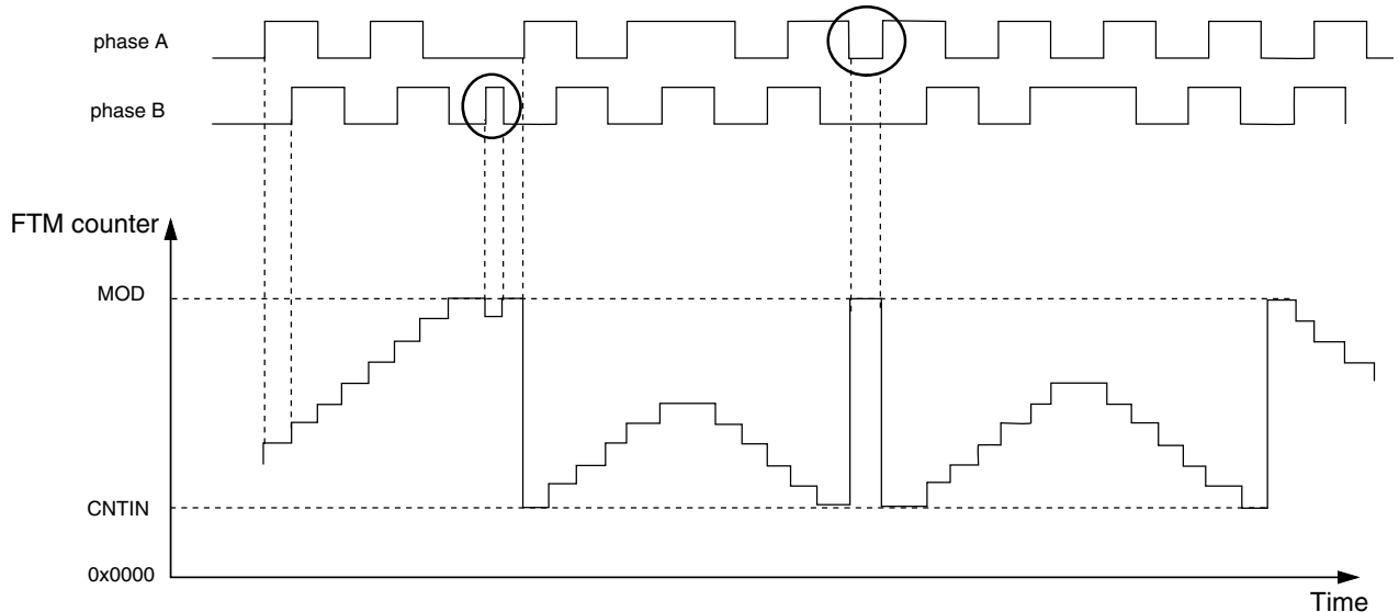
Figure 37-256. Motor Position Jittering Near Maximum and Minimum Count Value
