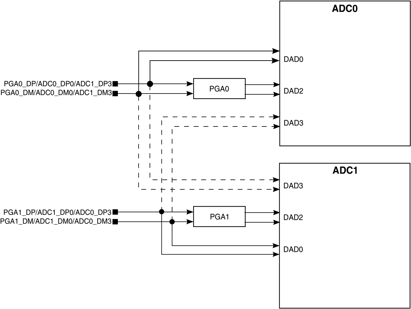
Figure 3-32. PGA Integration
