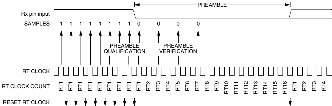
Figure 47-52. Receiver data sampling
