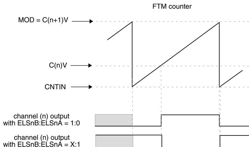
Figure 36-189. Channel (n) output if (CNTIN < C(n)V < MOD) and (C(n+1)V = MOD)
