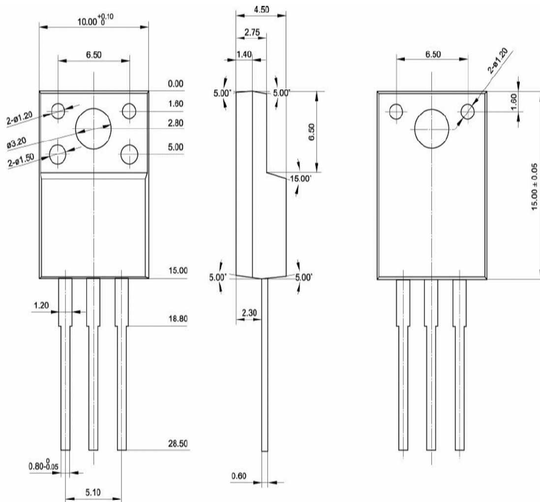
Fig.2 Outline dimensions
