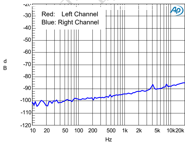
NOISE FLOOR
