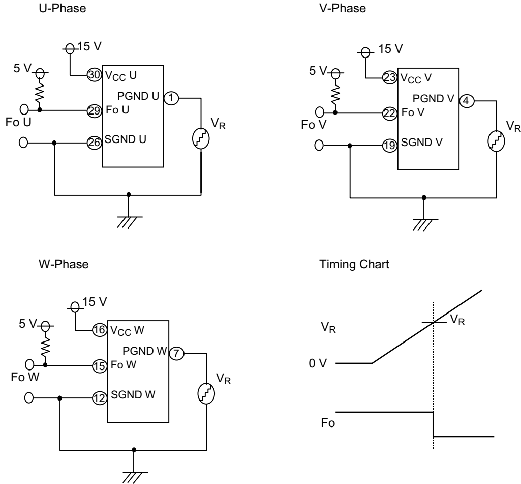
Note 2: V_R measurement circuit
