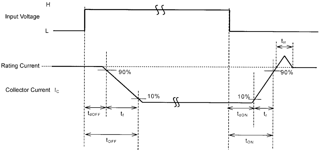
Note 3: Switching waveform
