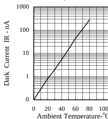
FIG.4 DARK CURRENT VS AMBIENT TEMPERATURE V_R=10 , E_e=0\text{ mw}/\text{cm}^2
