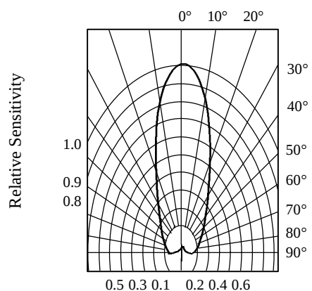
FIG.7 SENSITIVITY DIAGRAM
