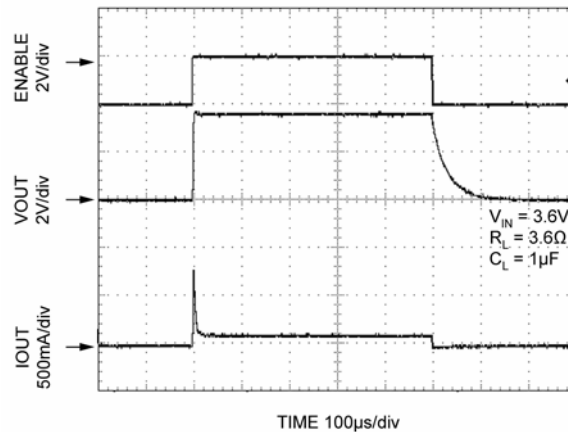
Turn-On/Turn-Off Timing
