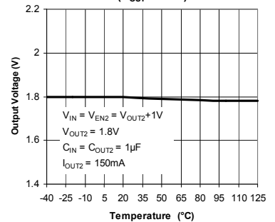
Output Voltage vs Temperature ( V_{OUT} = 1.8V )
