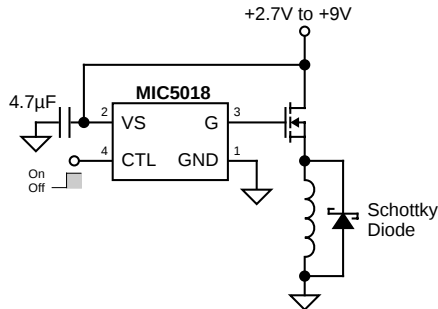
Figure 5. Switching an Inductive Load
