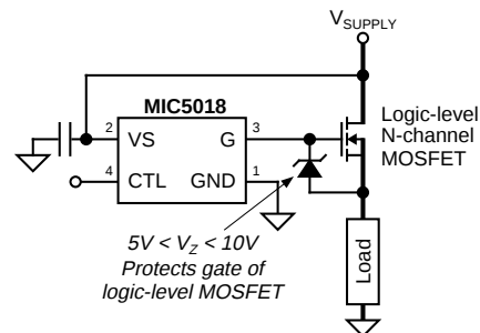
Figure 4. Gate-to-Source Protection
