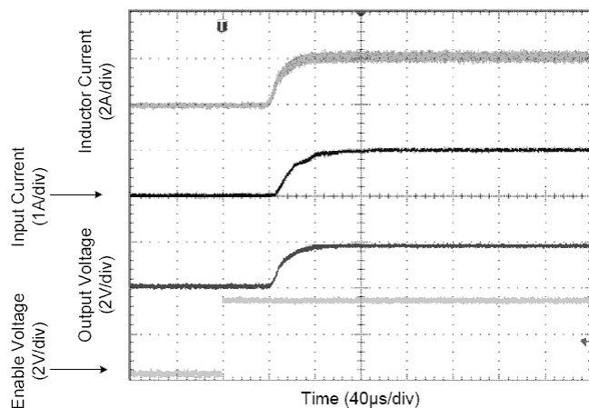
Start-Up Waveforms
