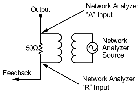
Figure 8. Transformer Injection
