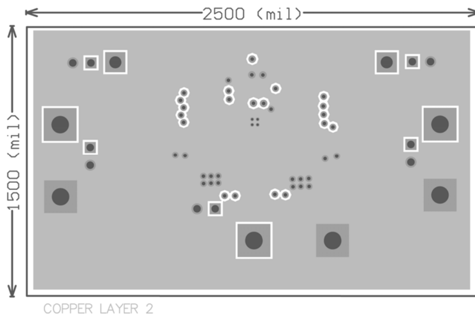
Mid-Layer 1
