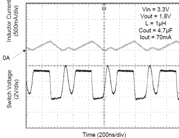
Discontinuous Current
