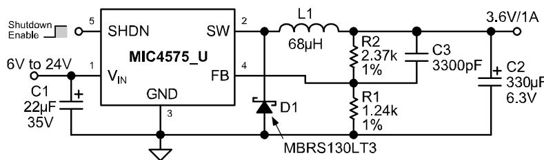
Adjustable Regulator
