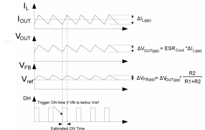
Figure 2. MIC28500 Control Loop Timing
