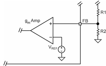
Figure 8. Voltage-Divider Configuration
