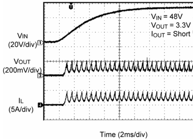
Short Circuit
