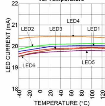
LED Current vs. Temperature
