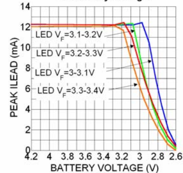
12mA Peak ILED vs. Battery Voltage
