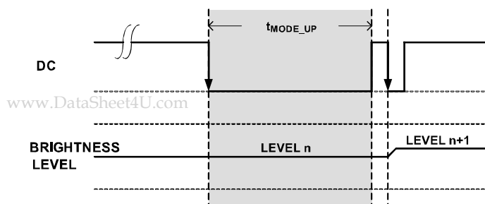
Figure 15. One-Step Brightness Increase
