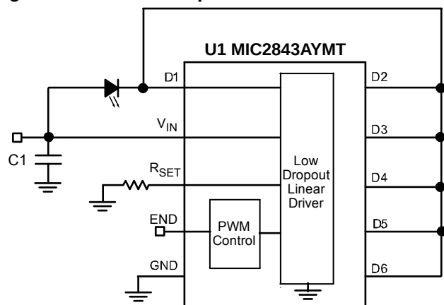
Figure 11. High Current LED Driver Circuit
