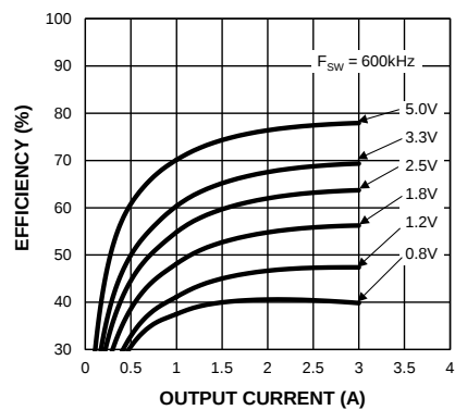
Efficiency (VIN = 38V) vs. Output Current (MIC28304-2)
