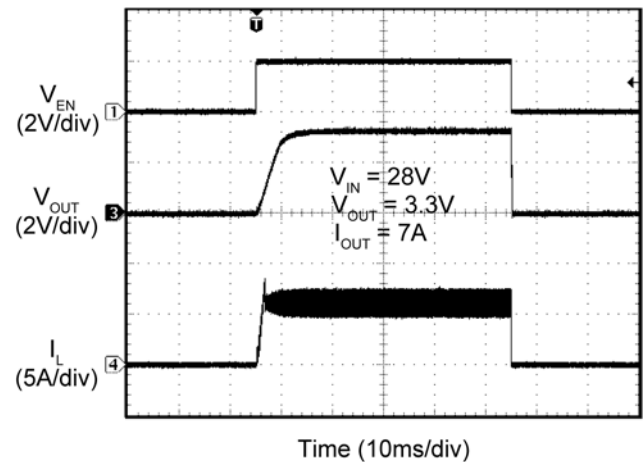
Enable Turn-On/Turn-Off
