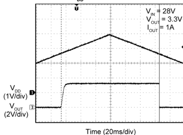
V_{DD} UVLO Thresholds
