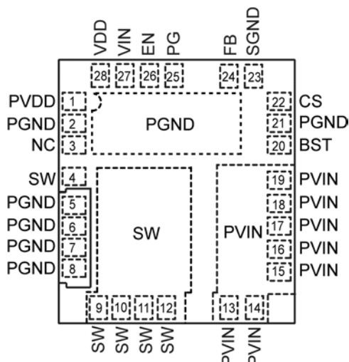
28-Pin 5mm x 6mm QFN (JL)
