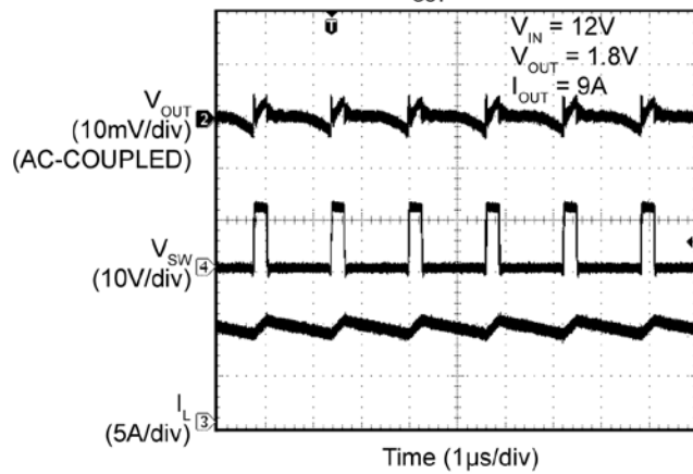
Switching Waveforms ( I_{OUT} = 9A )
