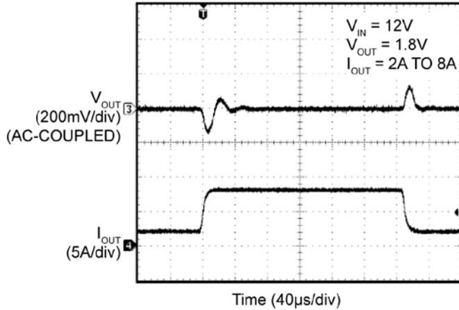
Transient Response
