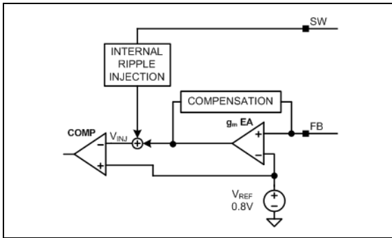
FIGURE 5-5: Internal Ripple Injection.
