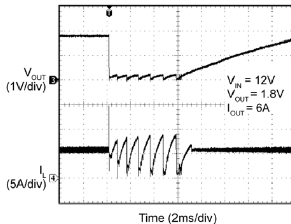
Output Recovery from Short Circuit
